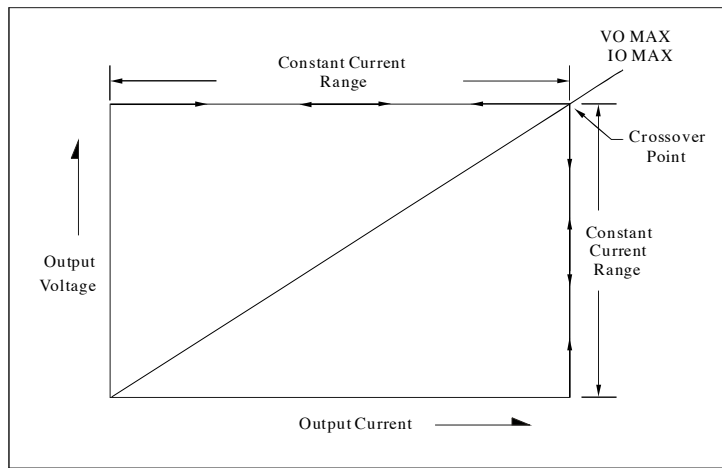
Fig.4-1 Constant Voltage/Constant Characteristic.
